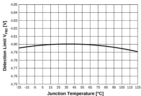
Figure 36 Detection Limit V_{FB2} vs. T_j
