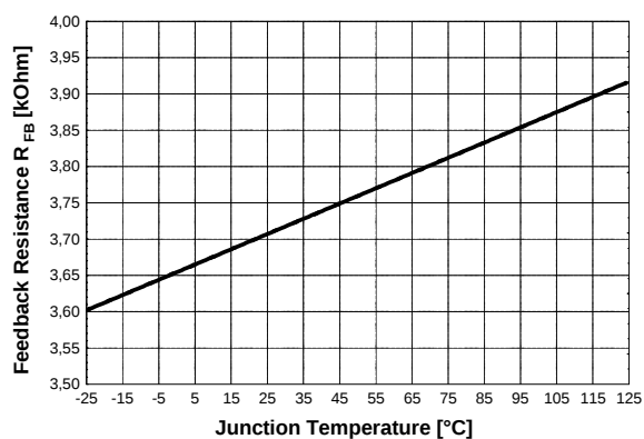
Figure 34 Feedback Resistance R_{FB} vs. T_j
