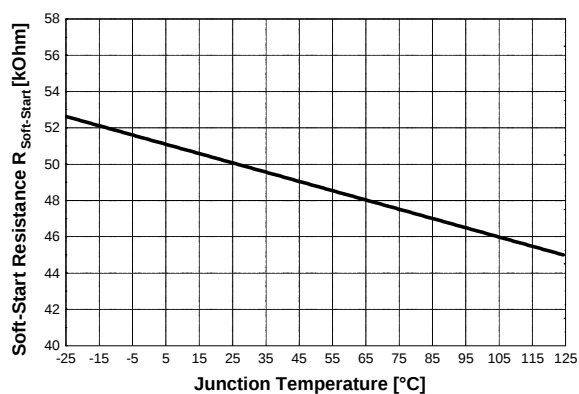
Figure 35 Soft-Start Resistance R_{Soft-Start} vs. T_j
